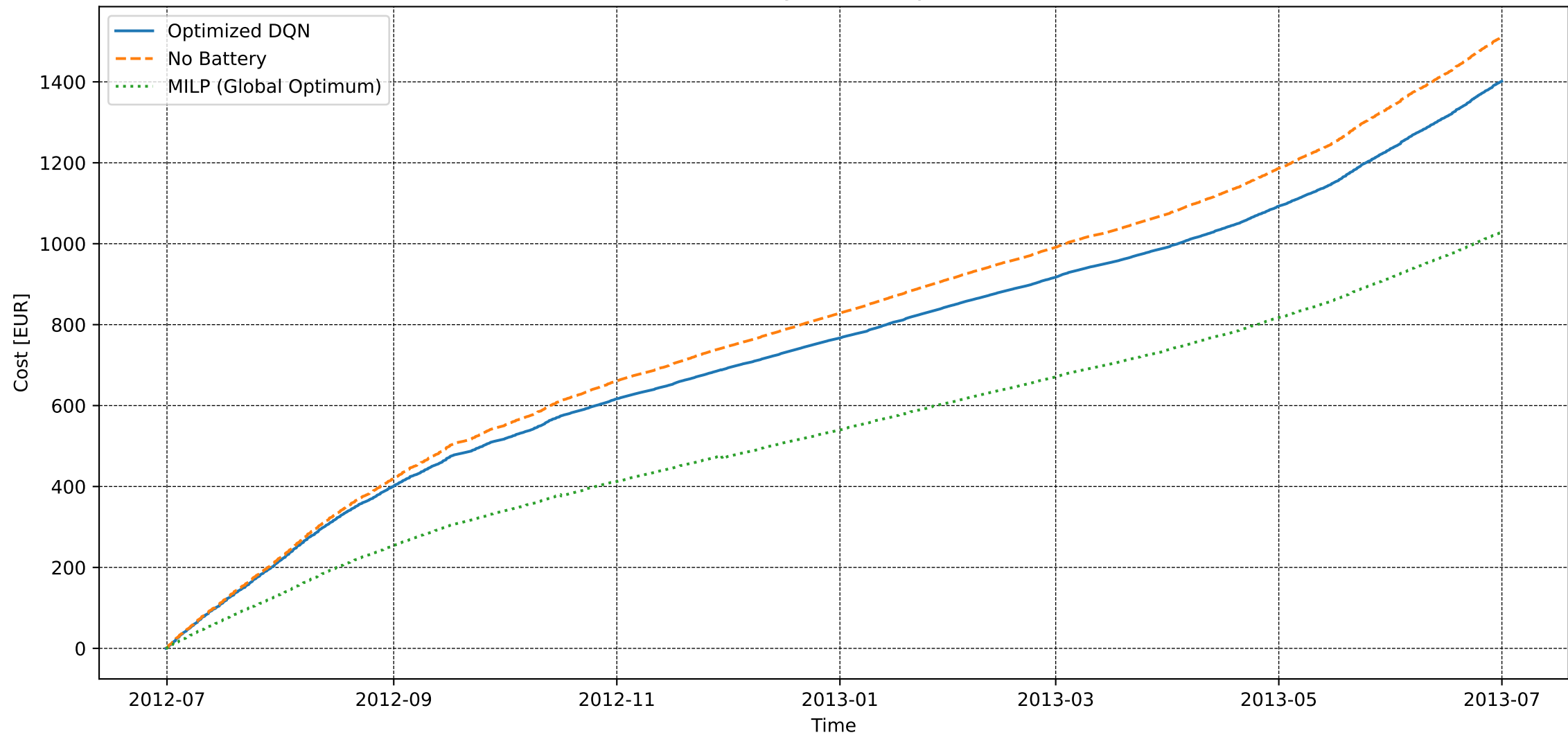
User 223 - Basic Training - Electricity Cost [DQN vs MILP]
